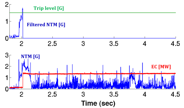
Fig. 4. Prompt suppression of the 3/2 NTM using Catch & Subdue. The real-time calculation of filtered NTM signals turned off after detection in this version of the control system. Normalized beta was controlled to a value of 2. The ratio j\text{ECCD}/j_{\text{boot}} was only 0.5 during the first NTM suppression at 2.2 seconds (partly due to high density) and then drifted up to 0.65 at 3.7 sec when a second (preemptive) NTM suppression occurred.
