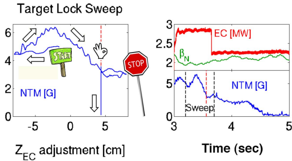
Fig. 2. Alignment correction with the Target Lock algorithm: a) left pane shows mode amplitude plotted versus adjustment of vertical position of the EC. The algorithm begins by moving quickly to -8 cm. The mode begins to rise and keeps rising until the adjustment is almost back at 0. When the adjustment goes to positive values the mode keeps decreasing but after +8 cm it levels off. The algorithm stops at +8 cm and decides that +4.4 cm is optimum since the mode was both small and decreasing there, b) right pane shows time traces of EC power, BN, and the NTM. After adjustment a gyrotron is lost leading to a drop in EC power and BN climbs to 2.15 at 4 seconds which delays the suppression.
