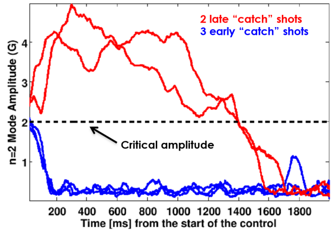
Fig. 5. Showing the 3/2 mode amplitude for 5 cases. The ECCD is turned on at t = 0 in all cases. For the cases shown in red the mode has then already exceeded the critical amplitude for prompt suppression which then takes significantly longer.
