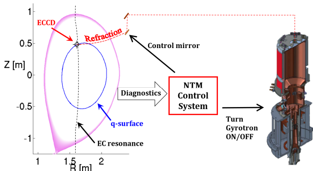
Fig. 1. The NTM control system analyzes diagnostics to detect NTMs and find positions of ECCD and q-surfaces. The beams from the gyrotrons are reflected by focusing mirrors and controlled steerable mirrors into the plasma where they are refracted by the plasma and absorbed at the EC resonance line to produce ECCD. The mirrors are typically controlled even when the gyrotrons are off so that the ECCD will be immediately aligned when the gyrotrons are turned on.
