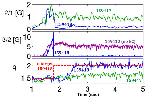
Fig. 3. Multi-mode control with all mirrors aimed at q = 1.5 and switching to q = 2 at 1.8 seconds. All mirrors moved almost exactly together. Top pane shows the 2/1 NTM in blue for shot 159418, also shown is the mode in the previous shot that had EC aimed at q = 3/2 for the entire shot. The middle pane shows the 3/2 mode for shot 159418 and for a shot without EC. The blue trace in the lower pane is the q at the ECCD point for 159418 and 159417. By targeting the 3/2 surface early and then the 2/1 surface, as in 159418, both modes were suppressed.
